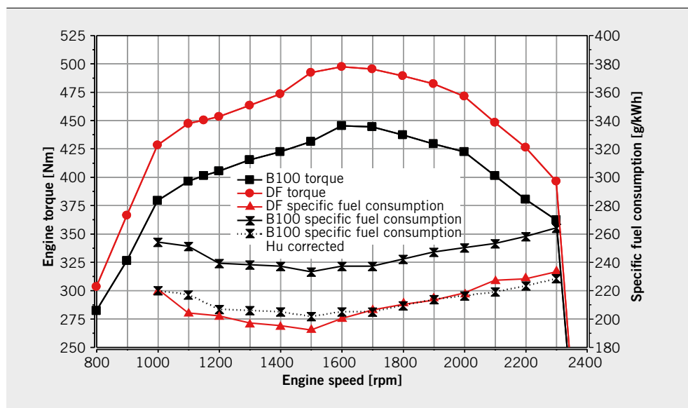
FIGURE 3 Torque curve and fuel consumption of DF and B100 (© Universität Rostock)
