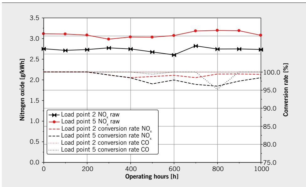
FIGURE 5 Nitrogen oxide concentrations and conversion rates throughout the operation time of 1000 h for B100 operation (© Universität Rostock)
