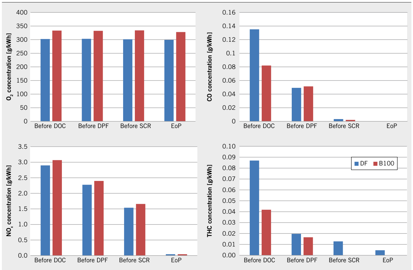
FIGURE 4 Exhaust gas concentrations for DF and B100 at load point 6 (n = 1,600 rpm, M = 370 Nm) (© Universität Rostock)
