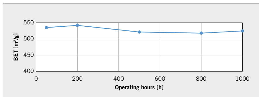
FIGURE 6 BET of the SCR throughout the operating time of 1000 h (© Universität Rostock)
