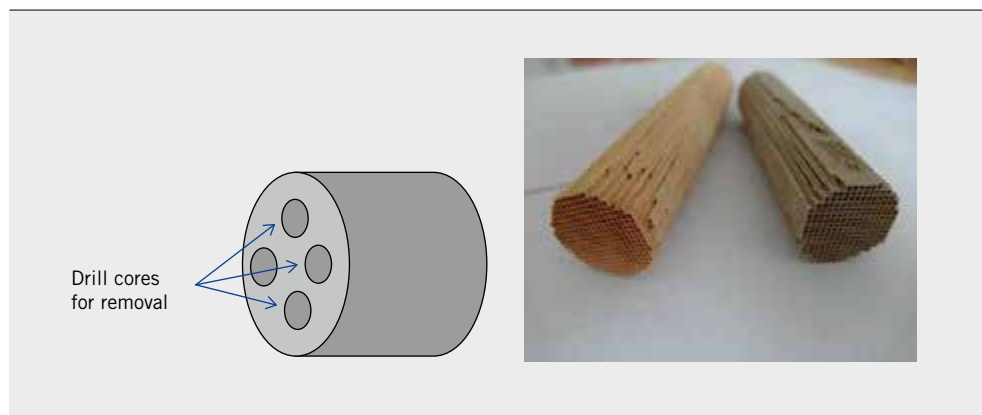
FIGURE 2 Representation of drill core removal and cores from the DOC and SCR (© Universität Rostock)
