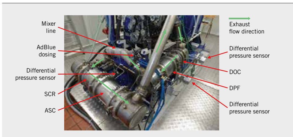
FIGURE 1 Setup of the exhaust aftertreatment system of the engine on the test bench (© Universität Rostock)
